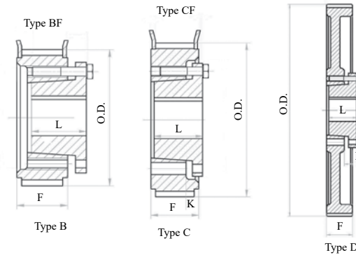
For belts 55MM wide * 14MM Pitch * Face Width (F) = 2 3/4"
