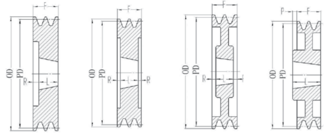
Type E Type F Type J Type G
