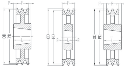
Type K Type M Type L
