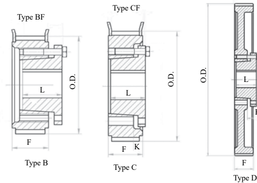
For belts 40MM wide * 14MM Pitch * Face Width (F) = 2 1/8"
