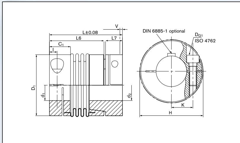
Sectional view PKA
