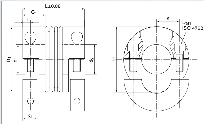
Sectional view AKN-H
