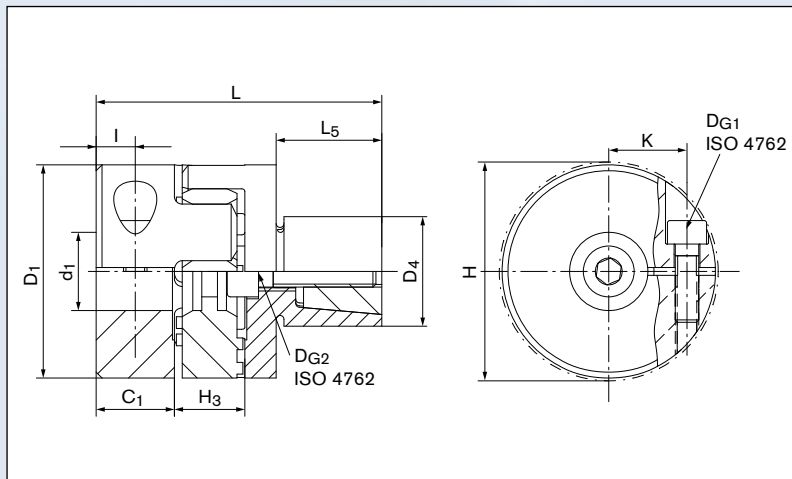
Sectional view GWE 5107
